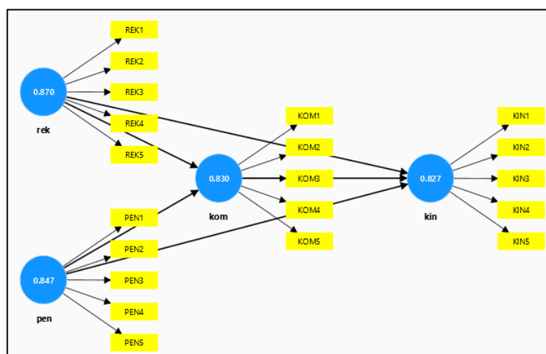
Figure 2. SEM-PLS Model
